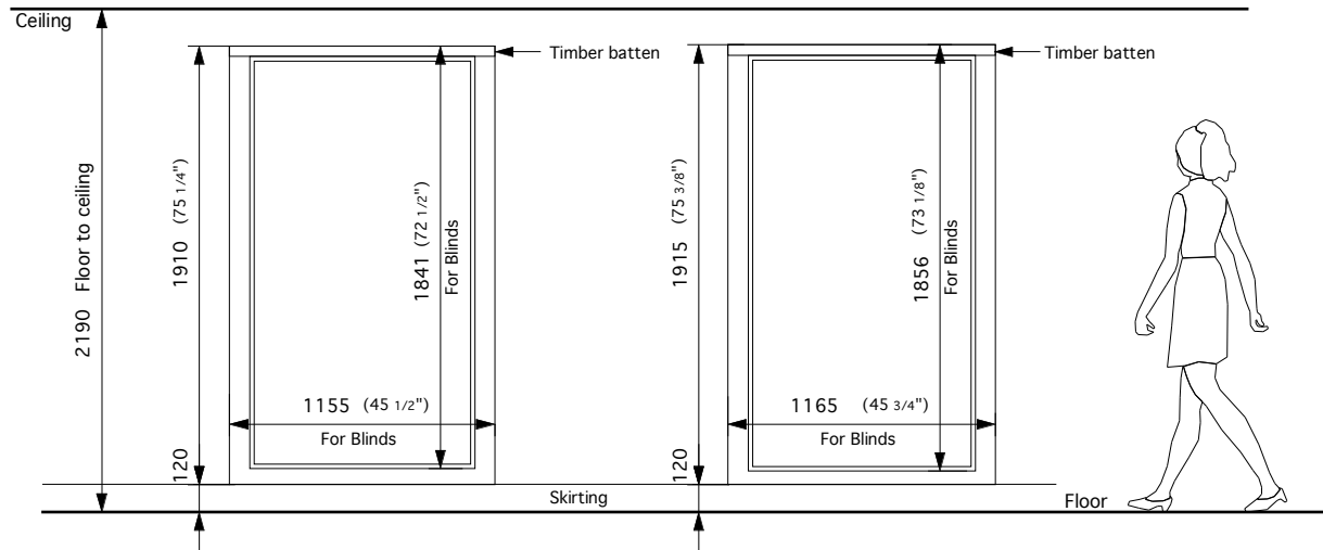
LOWER GROUND REAR Single vertical sliding sash window. Facing West.
