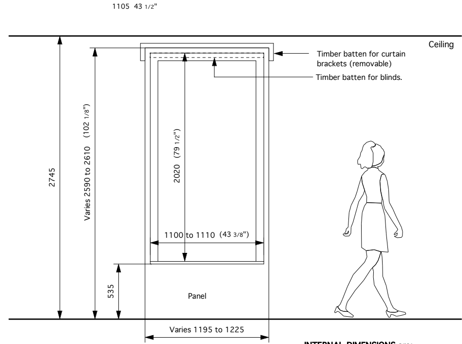
FIRST FLOOR FRONT AND REAR (4 no.) Single vertical sliding sash window. Facing south west.
