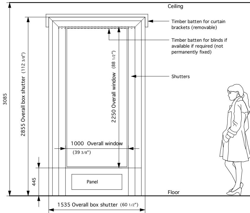
TYPICAL UPPER GROUND FLOOR BOX SHUTTER WINDOWS FRONT AND REAR (4 no.) Front and rear East and West Facing
