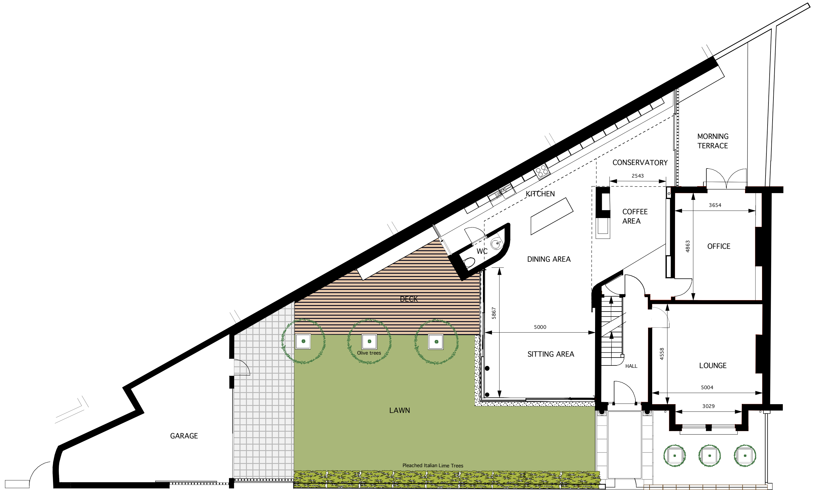
TEA ROOM - GROUND FLOOR PLAN 1:100 @ A3
